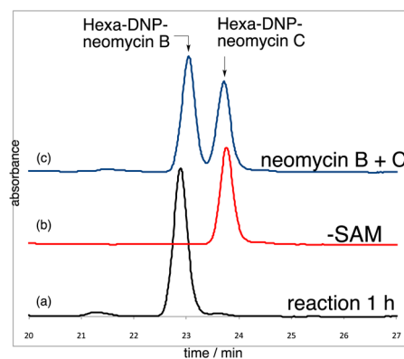
Figure 1. HPLC analysis (350 nm detection) of the NeoN reaction (1 h) with neomycin C and SAM: (a) NeoN (150 \mu\text{M} ) reaction with SAM (2 mM), neomycin C (1 mM), and \text{Na}_2\text{S}_2\text{O}_4 (10 mM) in a glovebox, (b) without SAM, and (c) the hexa-DNP derivative of neomycin B and C.
