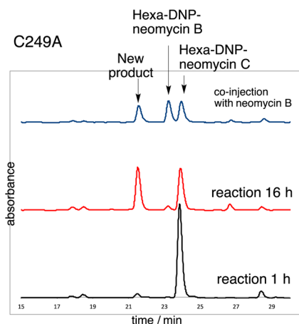
Figure 2. HPLC analysis (350 nm detection) of the C249A reaction with neomycin C and SAM: bottom, C249A reaction with SAM and neomycin C for 1 h; middle, for 16 h; top, co-injection of reaction mixture after 16 h with neomycin B.
