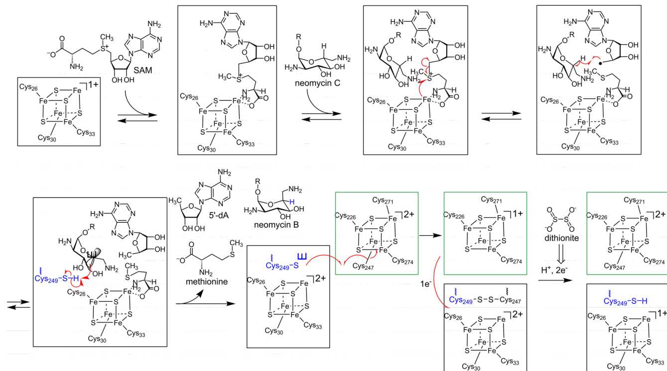
Scheme 3. Proposed NeoN Reaction Mechanism
